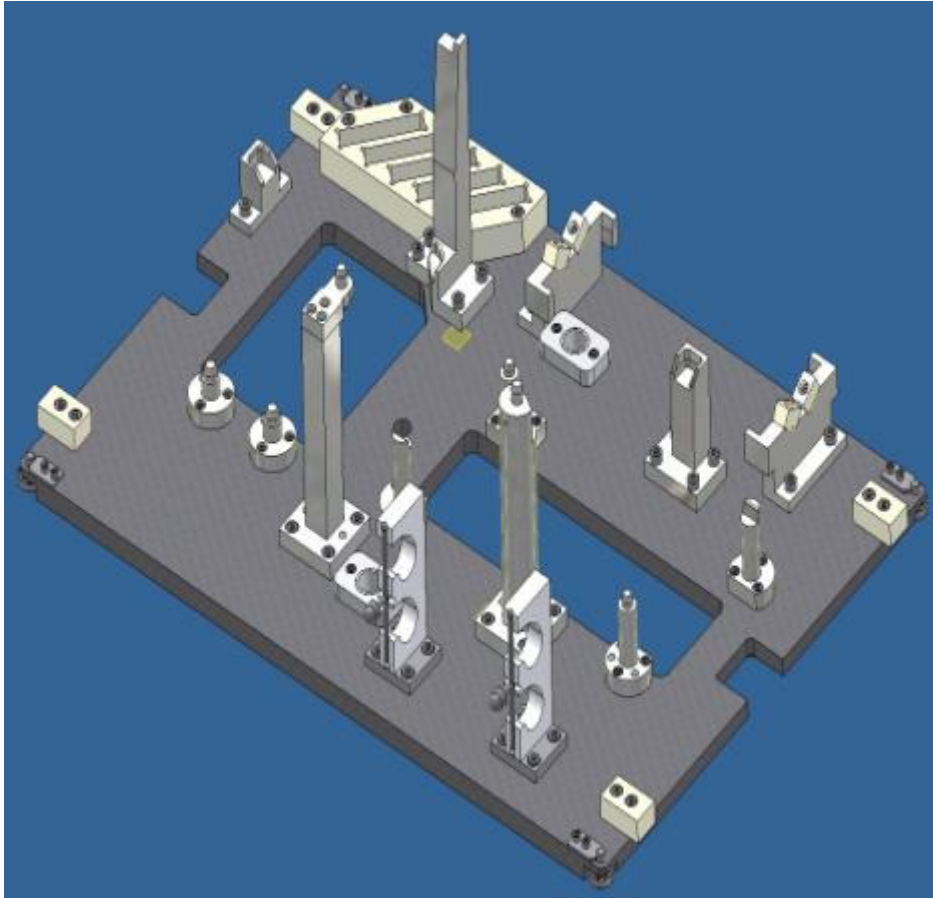
I20 KAPPA ENGINE ASSEMBLY FIXTURE
