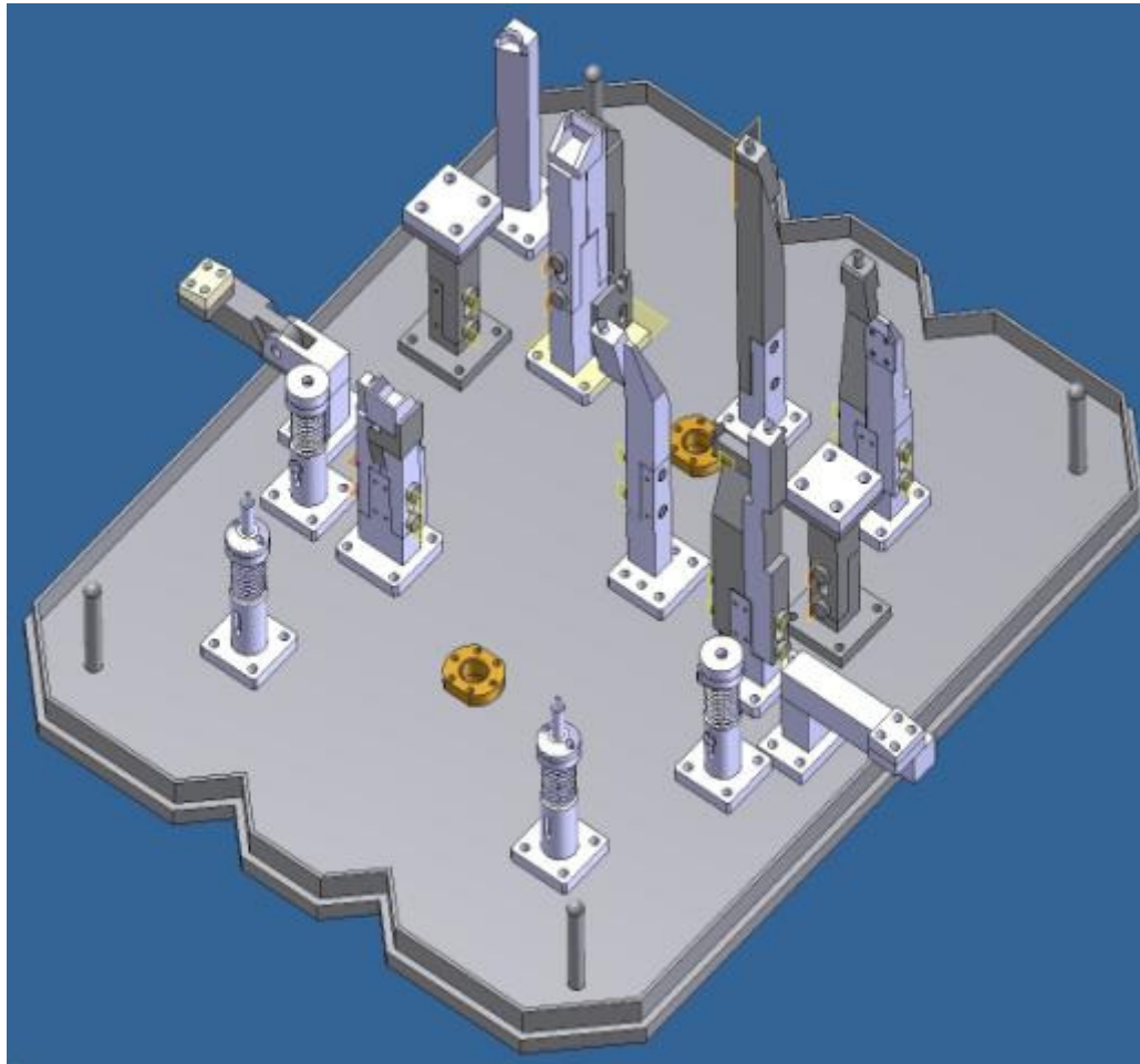
ACCENT FRT SUSP.ASSEMBLY FIXTURE
