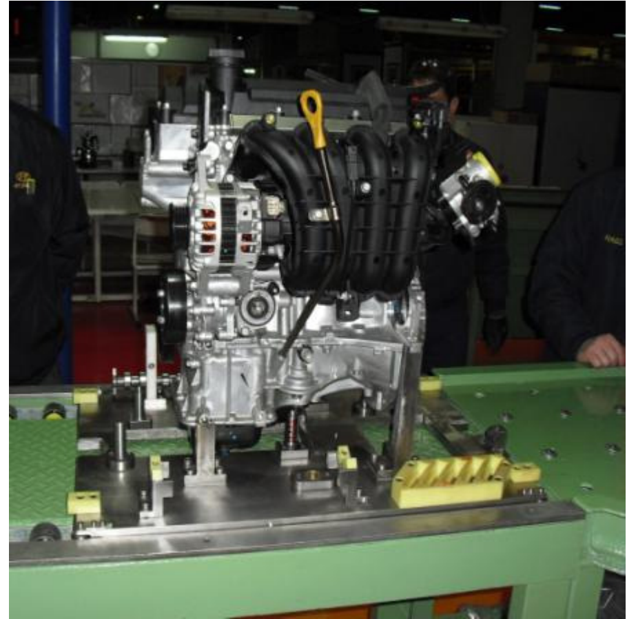
I20 KAPPA ENGINE ASSEMBLY FIXTURE
