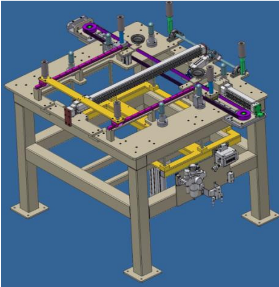
FRT GLASS SEALER FIXTURE
