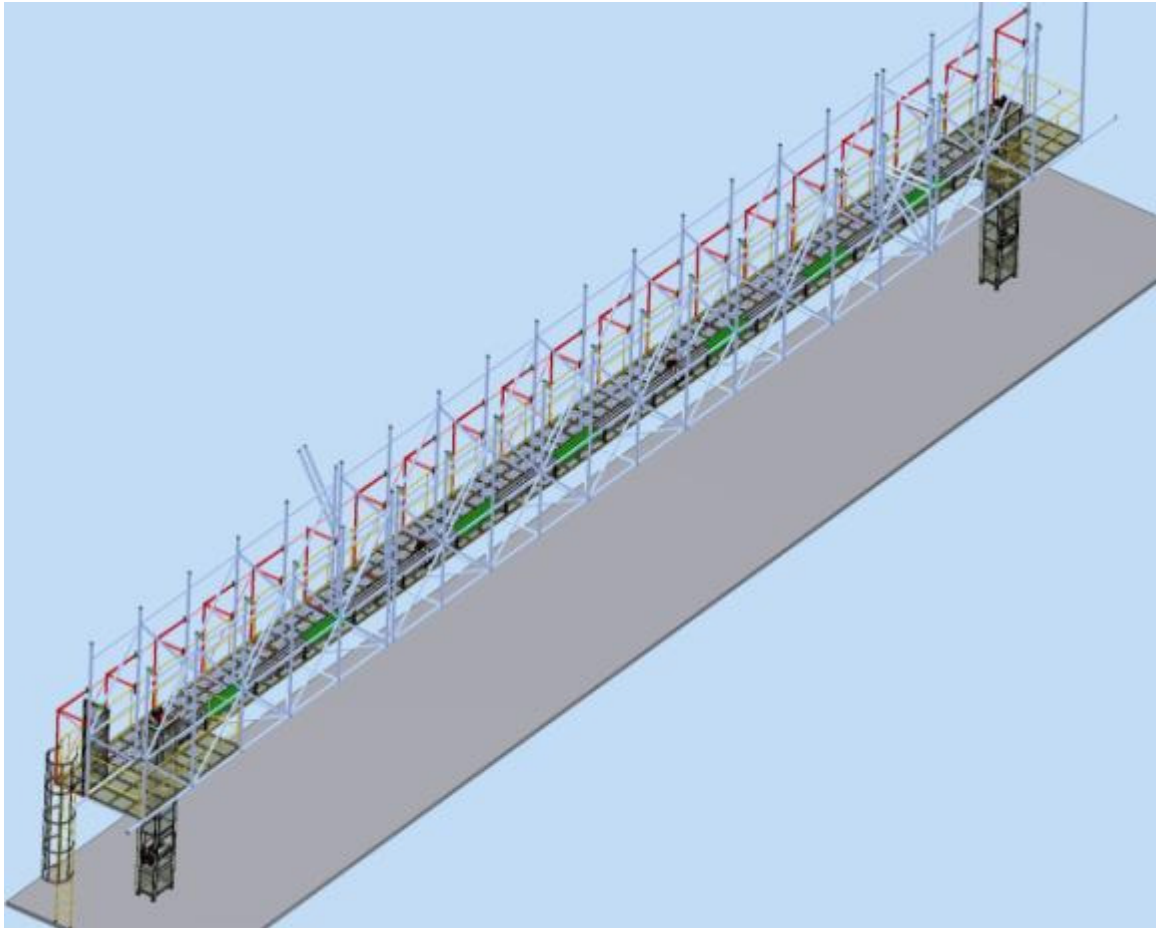
FORD ECAST TRANSFER CONVEYOR SYSTEM
