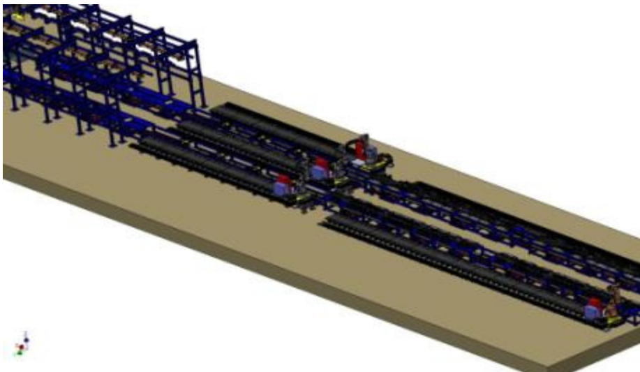
ULS TRAILER LONJERON WELDING LINE
